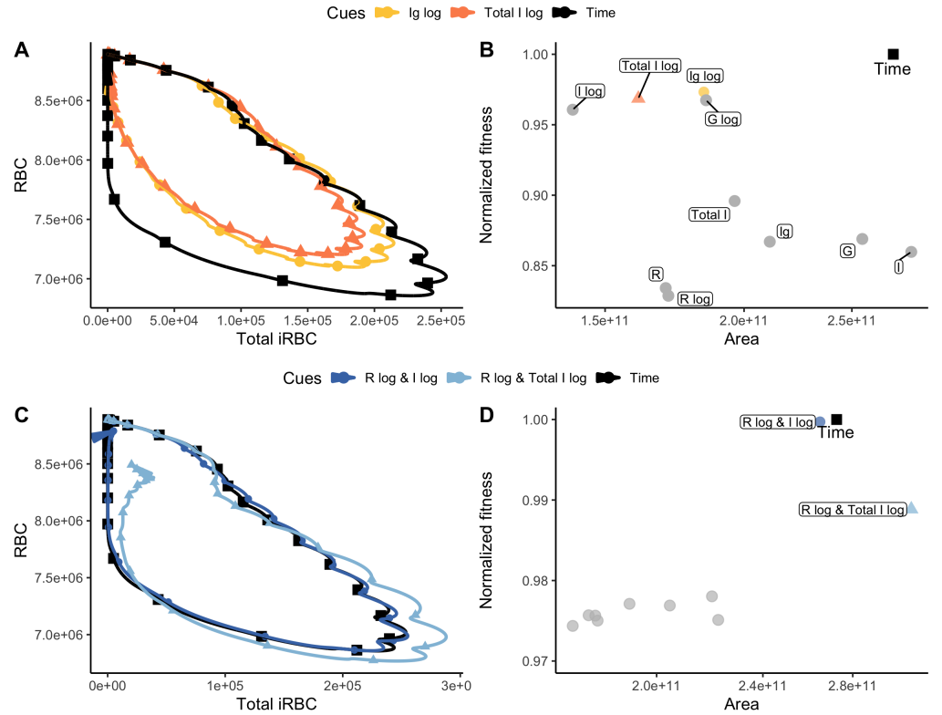
Fig 6. Cue perception mediates infection severity (virulence). (A, C) display the 30-day disease maps of infections where parasites adopt the top two optimal transmission investment strategies when sensing (A) a single cue or (C) dual cues. We use the area of the map traced as a proxy for virulence [46]. The trajectory of parasites that adopt the ideal transmission investment strategy (sensing time) is shown in black. (B, D) Relationship between disease map area and fitness (normalized with respect to the time-varying strategy) for parasites that sense (B) only one cue or (D) dual cues. The top two cues for single and dual cue perceiving parasites are coloured, while the grey points represent the other (B) single or (D) dual cues. Overall, these results suggest that perceiving only a single cue generates selection for strategies that lead to lower virulence while perceiving two cues generates selection for strategies that lead to higher virulence.
